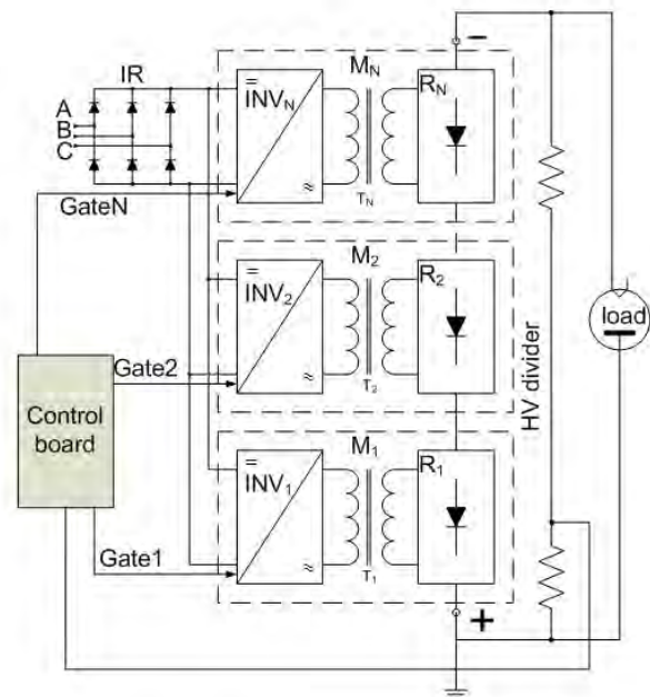
Fig. 1. HVPS block-diagram.
