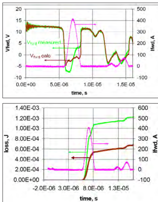
Fig. 9. FWD IXYS DSEI 2x61 losses. Plot a – green trace is measured signal; brown trace is V_{fwd} adjusted for inductive drop L di_{fwd}/dt (diode assembly inductance assessed at 5nH). Green and brown curves plot b match their counterparts in plot a. Divider Fig. 7, Floating scope.
