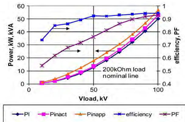
Fig. 12. Same as in Fig. 11 for 200-k \Omega load.
