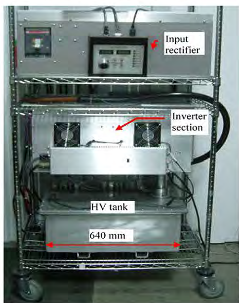
Fig. 5. Laboratory HVPS.
