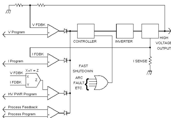
Fig. 2 Power Supply Control Loops
