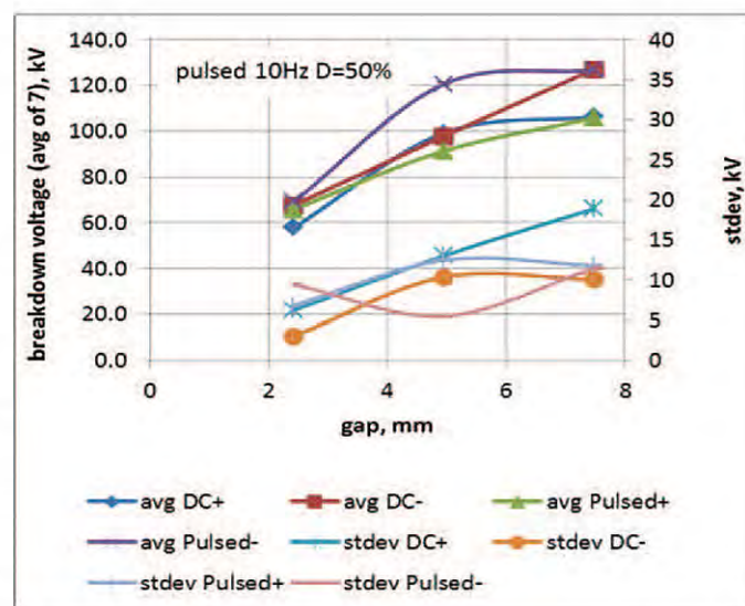
Figure 5. Breakdown voltages for fresh oil, without limiting resistors at the output of the cables. Pulse repetition rate (PRR) = 10Hz, D = duty cycle = 50%.
