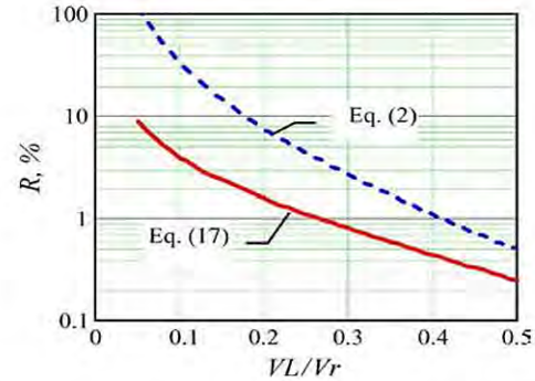
Fig. 9. Repeatability as a function of charge voltage, C_s = 200 nF, C1 = C2 = 2 \mu F, worst case.
